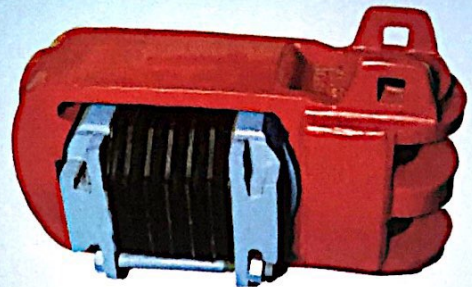
Draft Gear (for WDP4 HHP Locomotives)
