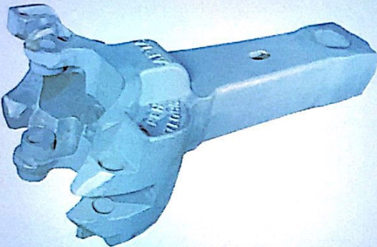
H-Type Tight Lock Coupler with F Type Shank (for Diesel & Electric Locomotives)
